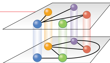
"SANDWICH" represents a graph of thickness two: two planar graphs in which the respective nodes have been stretched into vertical lines.
